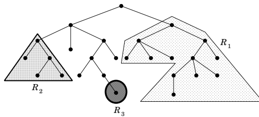
Figure 1: Semantic density
