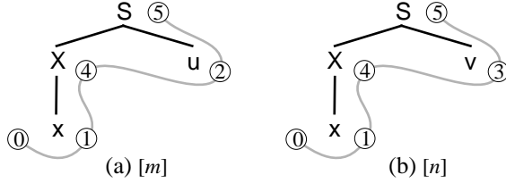
Fig. 1 Parse trees derived from grammar G1 (The square-bracketed value below each tree denotes the number of occurrences of that tree.)
