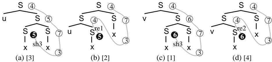
Fig. 3 Training set for grammar G3
